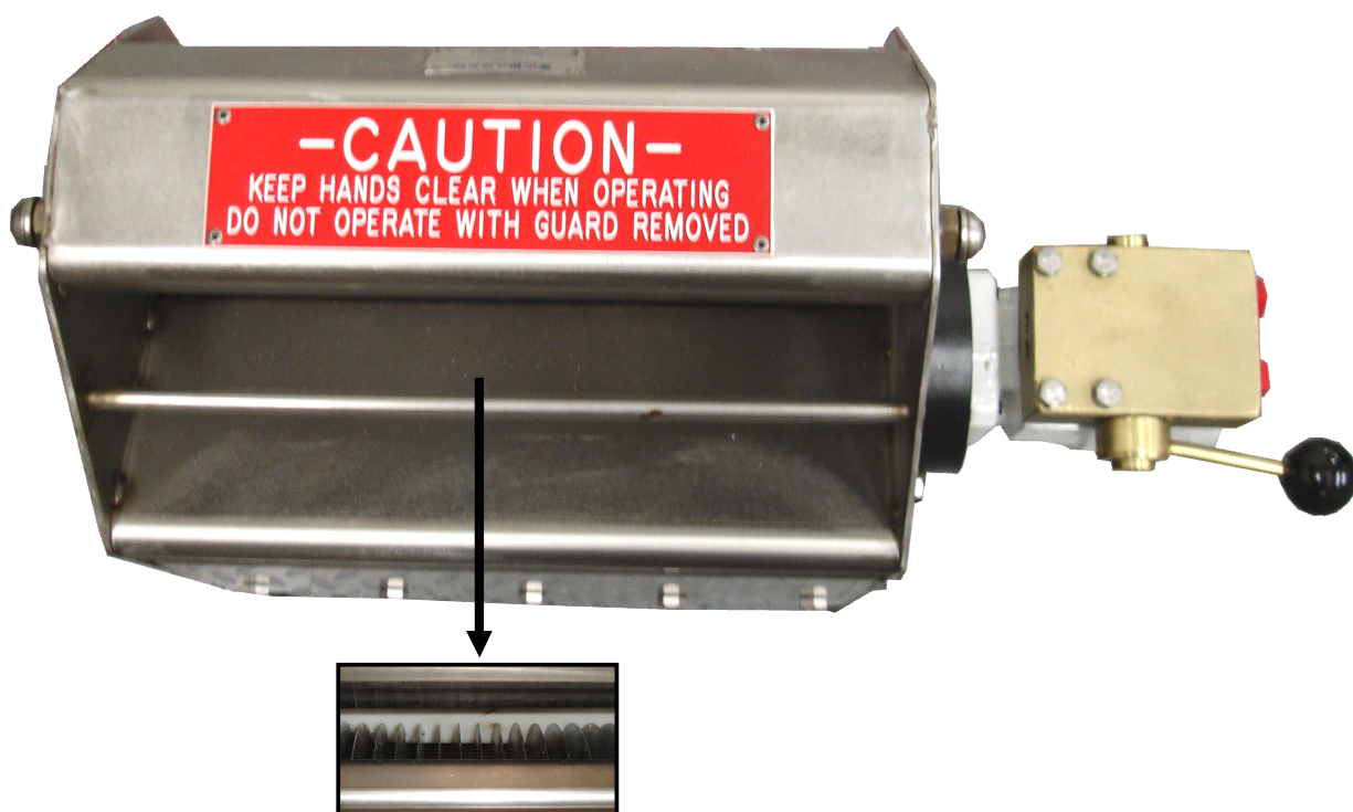
Blade Detail 5/8" Model with 19 Blades
